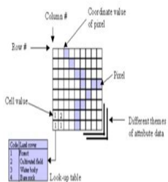
Figure 15: Characteristics of raster data structure
