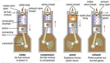
Four Stroke
